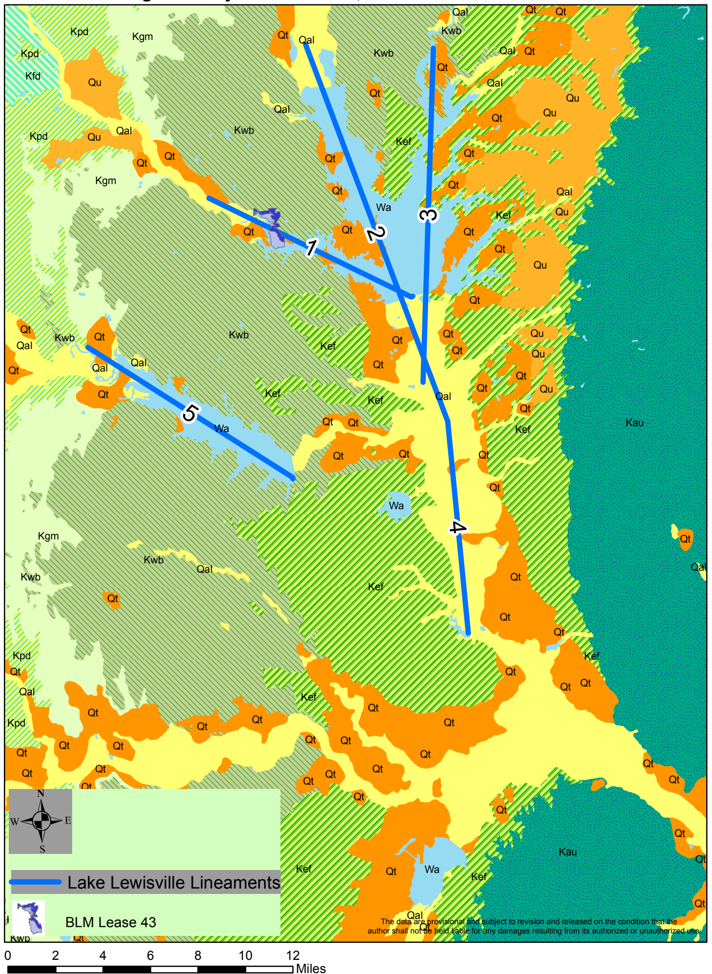
Figure 2 Major Lineaments, Lake Lewisville Area
