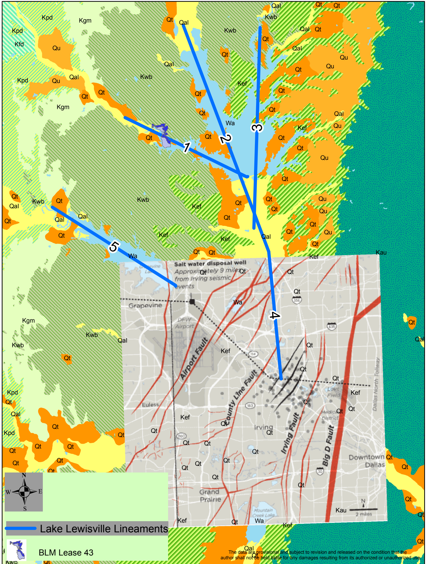
Figure 3 Major Lineaments, with XTO Faults and USGS Earthquakes (dots)
