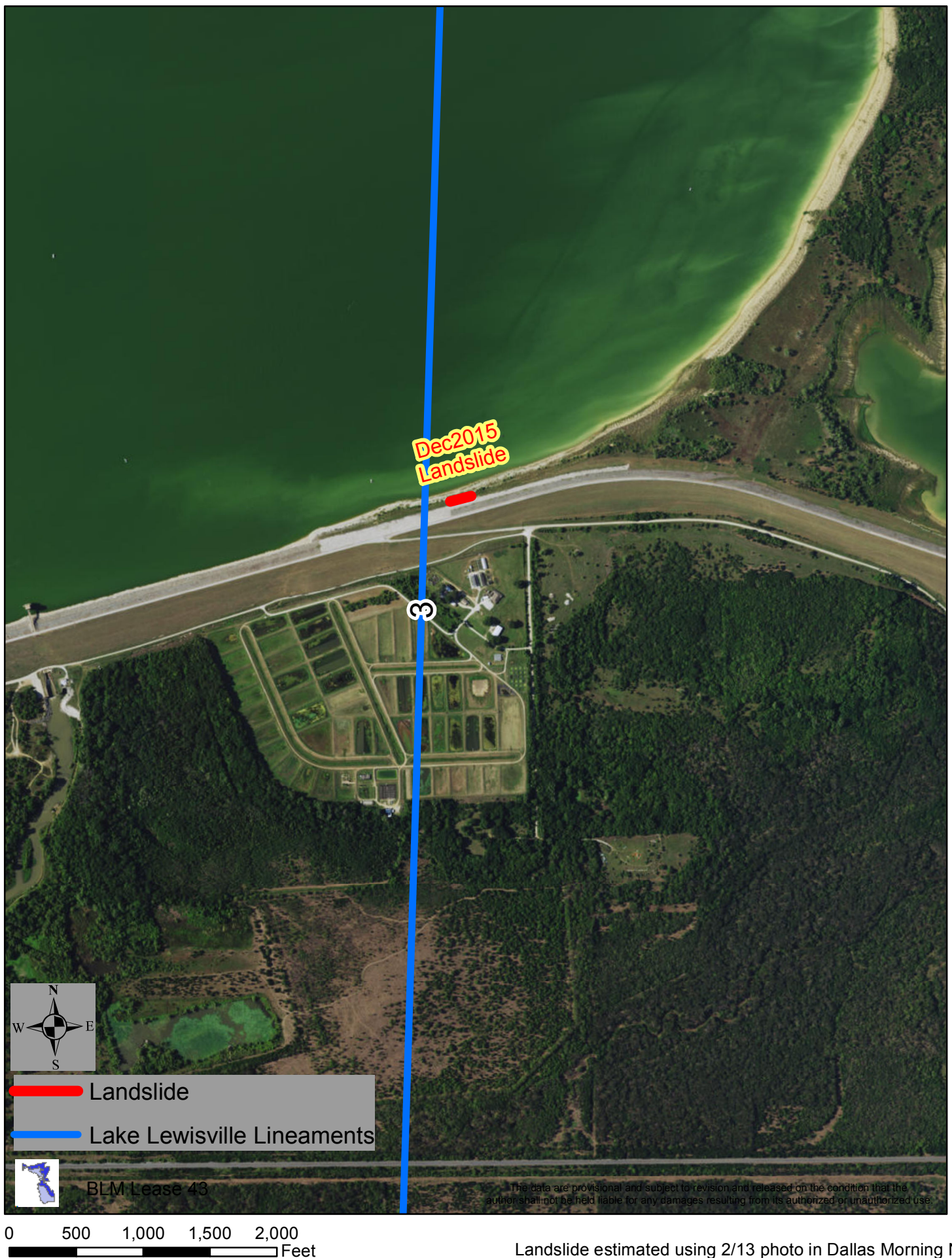
Figure 4 Relationship Between Lineament and Location of December 2015 Landslide, Lake Lewisville Dam
